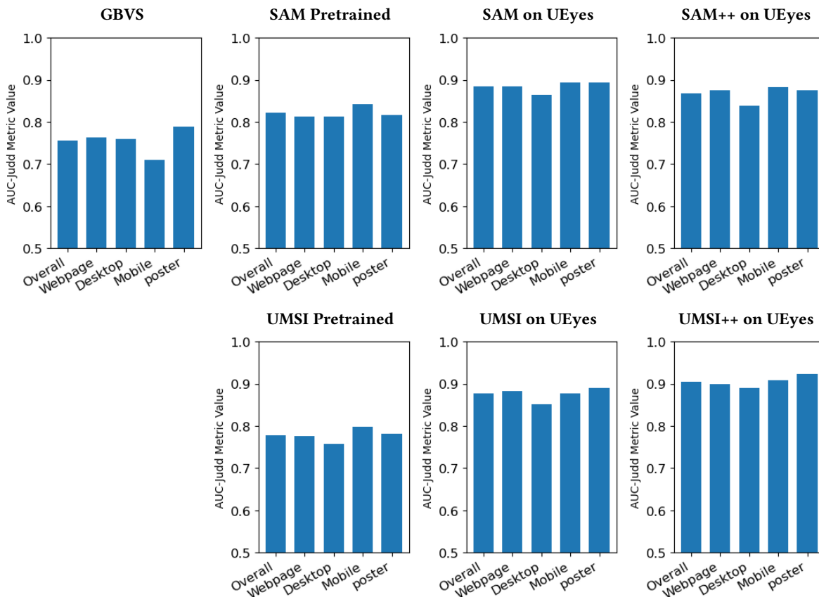
Figure 9: Comparison of saliency map models’ predictive accuracy, with AUC-Judd (designed to measure saliency map performance) as the metric. Larger values indicate higher accuracy. The figure shows that UMSI++ performs best across all the UI types.
